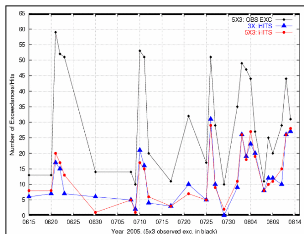
Fig. 2a. 8 hour 5x3 vs. 3x, correctly predicted/ observed events, June 15 - August 13, 2005, 935 stations.
