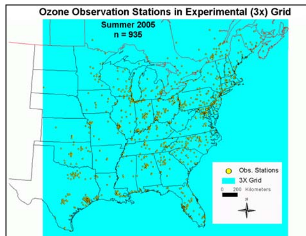
Fig. 1. 3x grid over the eastern U.S., 935 stations, 2005.
