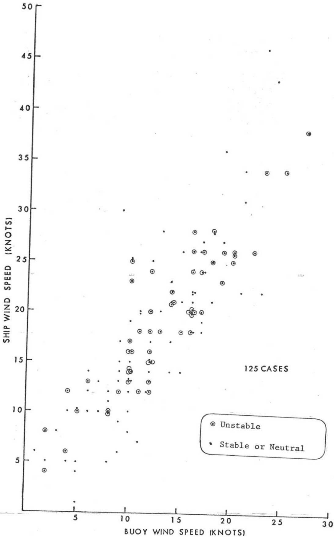
Figure 5. Plot of observed wind speeds at Great Lakes data buoys and the corresponding wind speeds observed on nearby ships. Unstable cases, where the air-water temperature difference is less than -2.8^{\circ}\text{C} , are circled.
