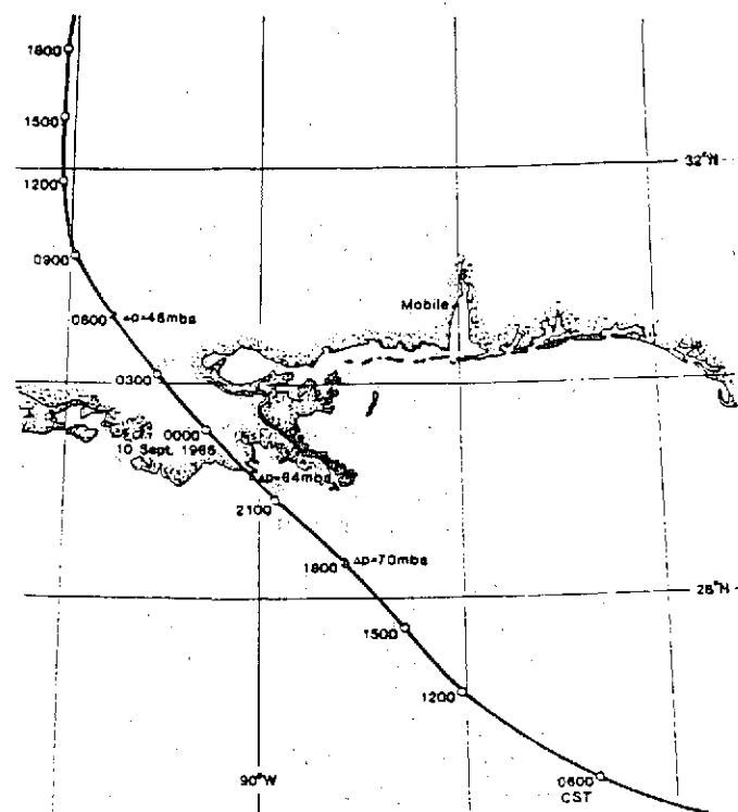
Figure 21. Meteorological input parameters for Hurricane Betsy, 1965.
